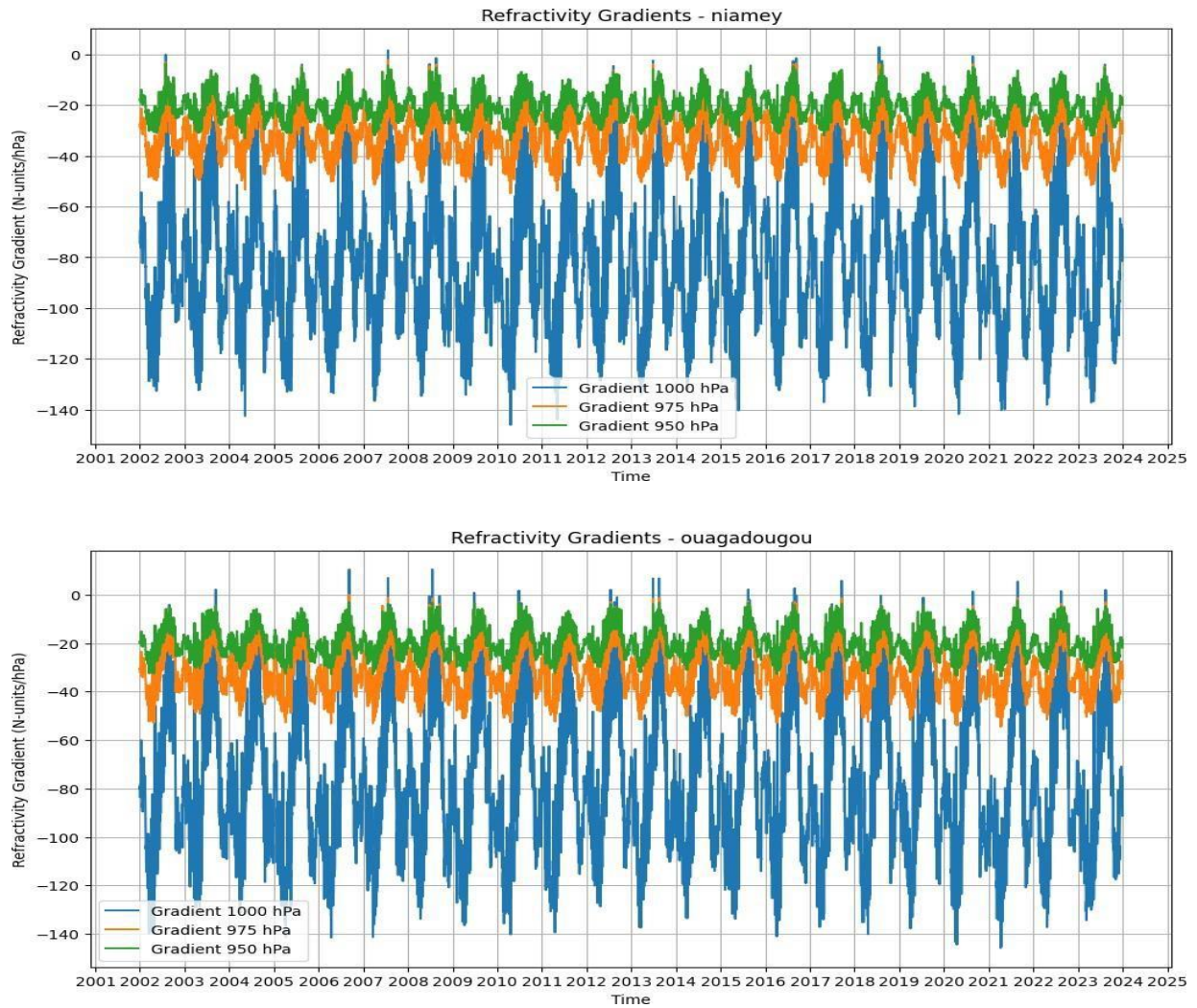
Figure 9a & 9b: "Refractivity gradient profiles in desert zones: (a) Niamey and (b) Ouagadougou, with strong gradients at 1000 hPa
