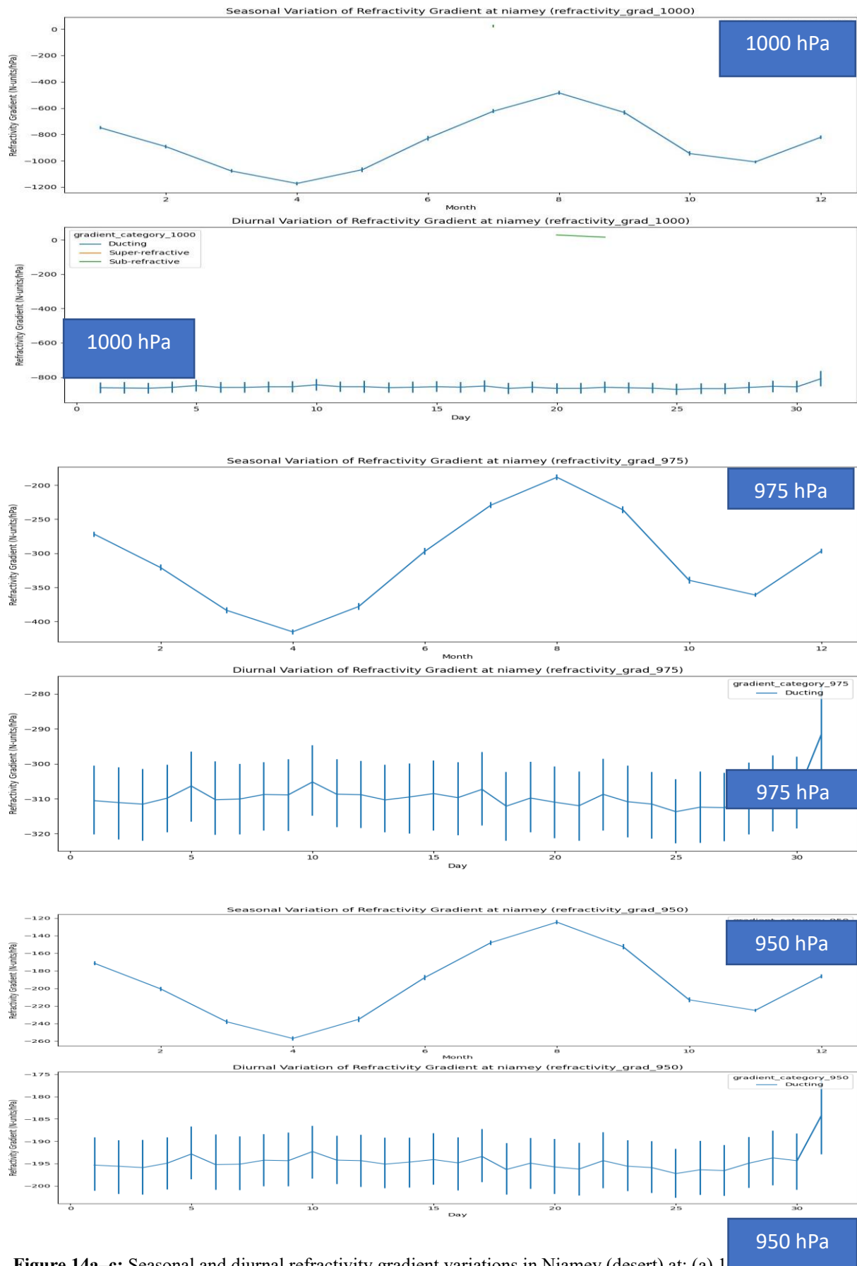
Figure 14a–c: Seasonal and diurnal refractivity gradient variations in Niamey (desert) at: (a) 1000 hPa, (b) 975 hPa, and (c) 950 hPa
