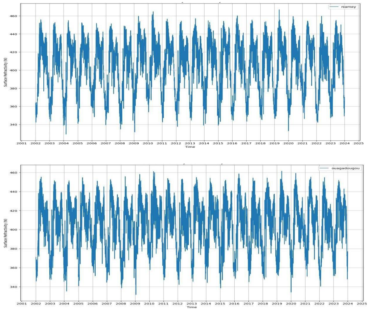
Figure 4a & 4b: Surface refractivity time series in desert zones: (a) Niamey and (b) Ouagadougou, with minima in 2015
