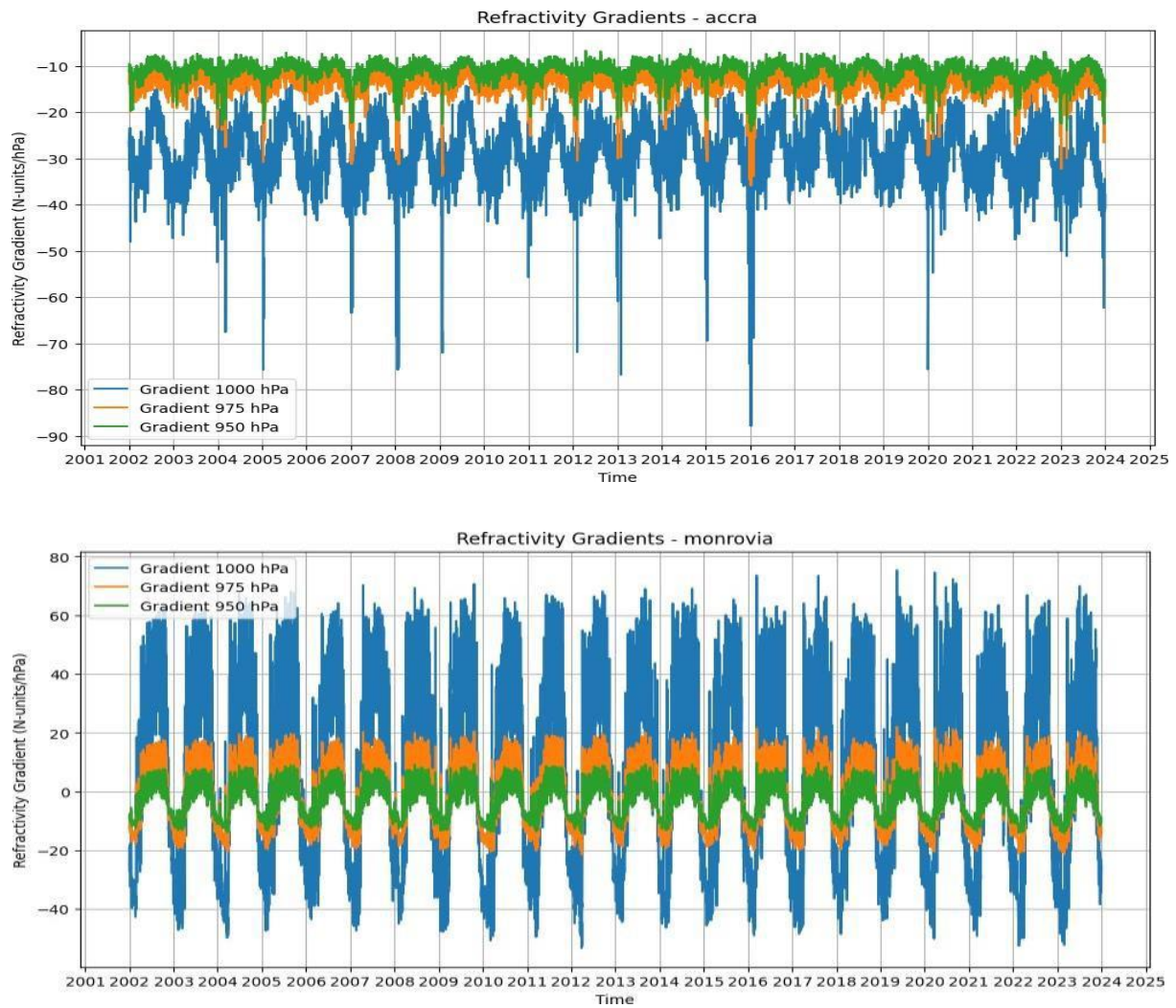
Figure 7a & 7b: Refractivity gradient profiles in coastal zones: (a) Accra and (b) Monrovia, showing altitude-dependent trends
