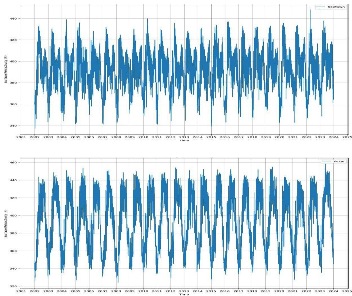
Figure 5a & 5b: Surface refractivity time series in coastal zones: (a) Freetown and (b) Dakar, reflecting stable maritime influence
