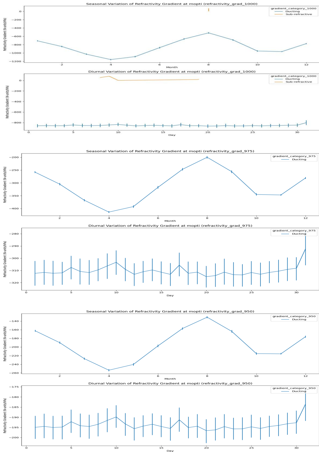
Figure 13a–c: Seasonal and diurnal refractivity gradient variations in Mopti (savanna) at: (a) 1000 hPa, (b) 975 hPa, and (c) 950 hPa
