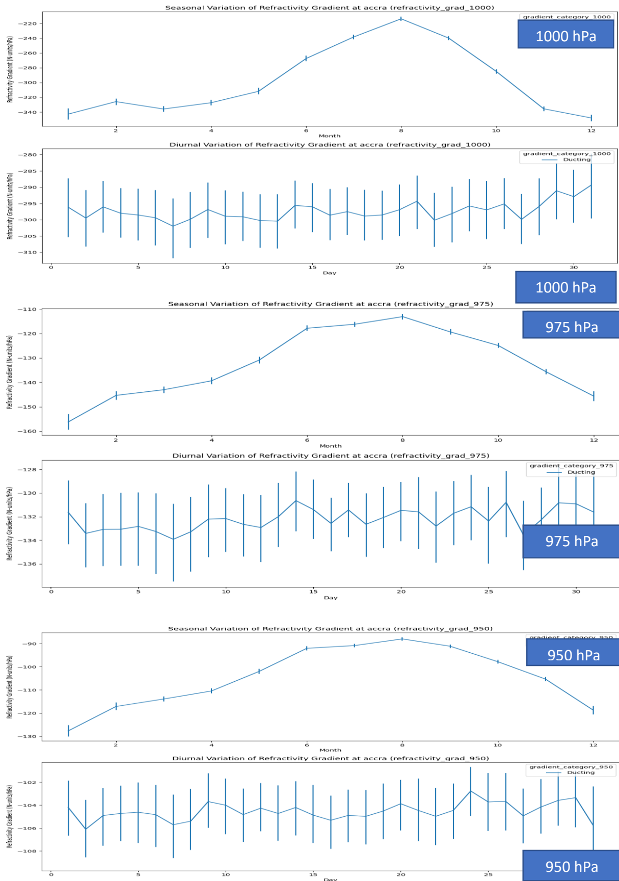
Figure 12a-c: Seasonal and diurnal refractivity gradient variations in Accra (coastal) at: (a) 1000 hPa, (b) 975 hPa, and (c) 950 hPa
